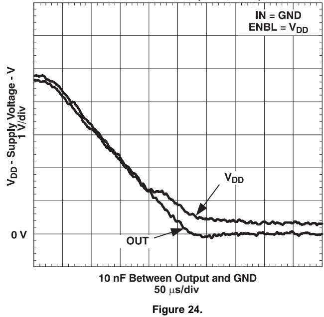
OUTPUT BEHAVIOR vs VDD (INVERTING)
